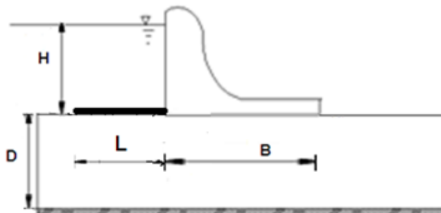
Figure (2): Blanket Model
