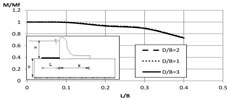
Figure (6): The Effect Of The Length Of The Blanket On The Moments Of The Lifting Forces Under The Concrete Dams
