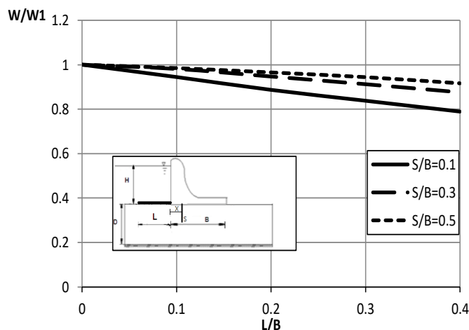
Figure (9): Comparison Between The Effect Of Using The Blanket And Using The Front Cutoff On The Lifting Forces Under Concrete Dams
