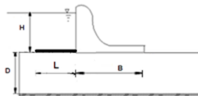
(B) Use Of An Impermeable Blanket
