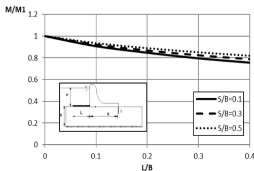
Figure (14): Comparison Between The Effect Of Using The Blanket And Using The Back Cutoff On The Lifting Force Moments Under Concrete Dams
