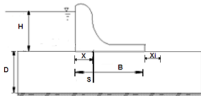
(A) Use Of Cutoff
