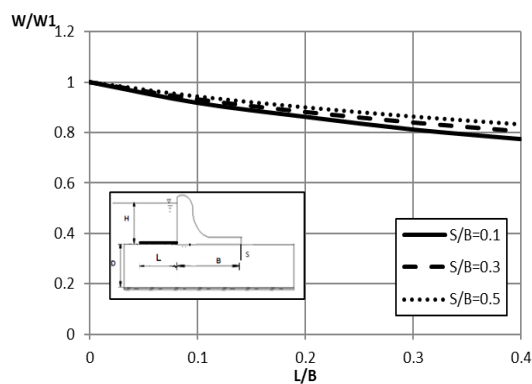
Figure (13): Comparison between the effect of using the blanket and using the back cutoff on the lifting forces under concrete dams .
