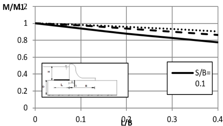
Figure (10): Comparison Between The Effect Of Using The Blanket And Using The Front Cutoff On The Lifting Force Moments Under Concrete Dams
