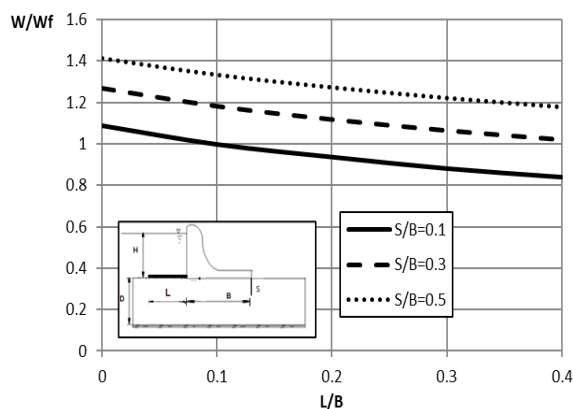
Figure (11): The effect of the length of the blanket on the lifting forces under concrete dams in the presence of a back cutoff
