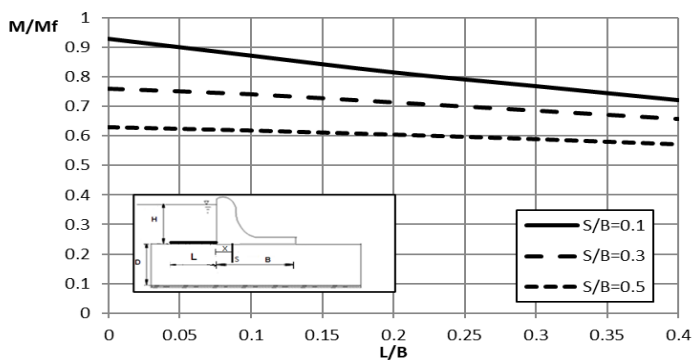
Figure (8): The Effect Of The Length Of The Blanket On The Moments Of The Lifting Forces Under The Concrete Dams In The Case Of The Presence Of A Front Cutoff.
