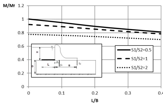
Figure (15): The Effect Of The Length Of The Blanket On The Moments Of The Lifting Forces Under The Concrete Dams In The Case Of The Presence Of Two Front And Back Cutoffs
