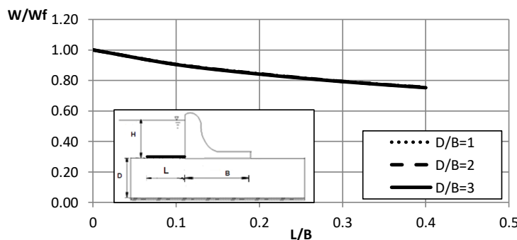
Figure (5): The Effect Of The Length Of The Blanket On The Lifting Forces Under The Concrete Dam
