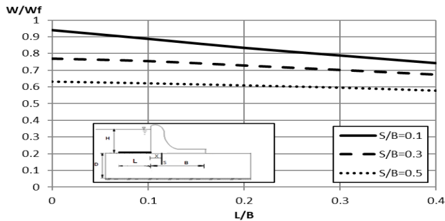
Figure (7): The effect of the length of the blanket on the lifting forces under concrete dams in the presence of a front cutoff.
