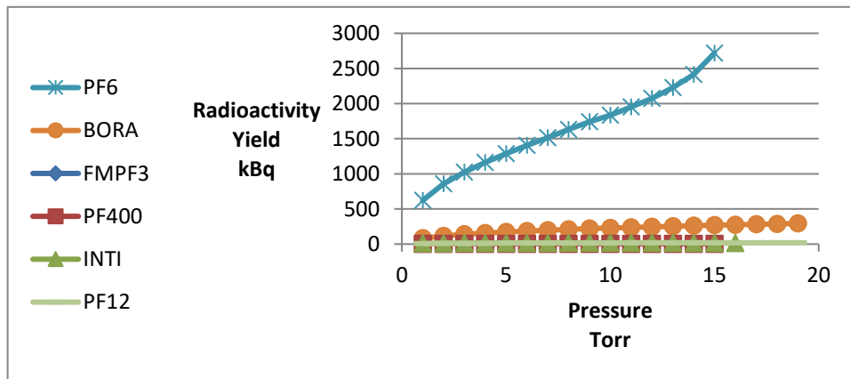
FIGURE (4): The values of the radiation yield of the studied devices at different values of deuterium gas pressure
