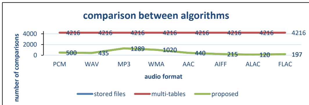
FIGURE (7): The Change In The Number Of Comparisons
