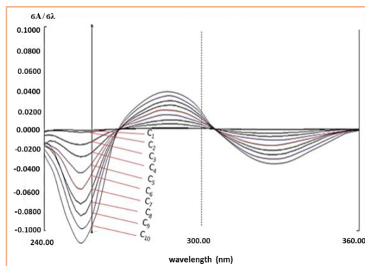
Figure (4): spectra of (Dic.Na):
