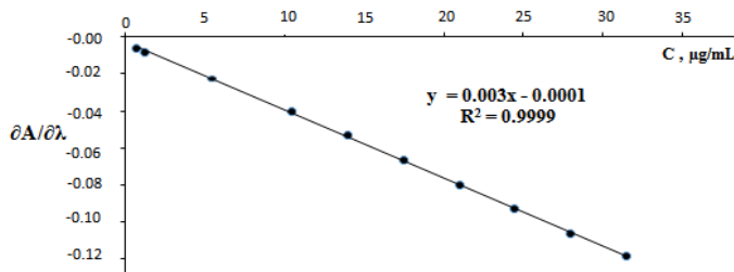
Figure (5): Calibration curve for (Dic.Na).
