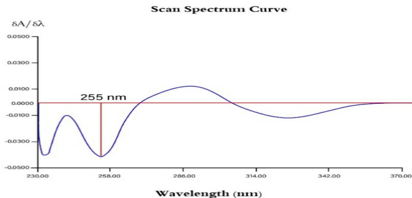
Figure (3): First derivative spectra, (Dic.Na) [12] \mu\text{g/mL} .
