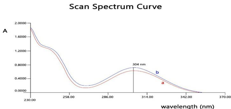
Figure (2): Zero spectrophotometric spectra, (Dic.Na) [12] \mu\text{g/mL} for both. a: standard (Dic.Na) and b: product sample (Dic.Na).
