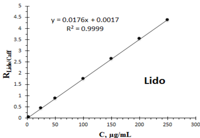
FIGURE (5): Linear Relationship For (LIDO): C 1 : 2.5 µG/ML, C 2 : 25 µG/ML, C 3 : 50 µG/ML, C 4 : 100 µG/ML, C 5 : 150 µG/ML, C 6 : 200 µG/ML, C 7 : 250 µG/ML. N = 5 FOR EACH CONCENTRATION.
