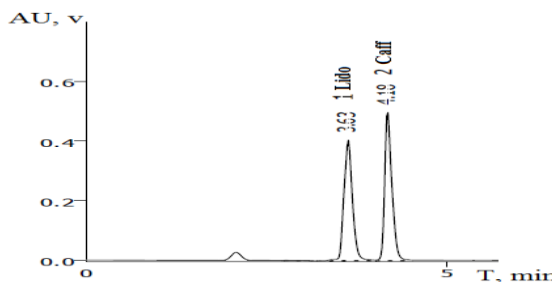
FIGURE (6): Chromatogram Of "OBARCAINE" VIAL: 1-(LIDO), 2- (CAFF) as internal standard 25 µG/ML. chromatographic conditions: C 8 column; mobile phase: acetonitrile:phosphoric acid (PH = 3) 30:70 (V/V); FLOW RATE 1.0 ML/MIN, temperaturE 30 °C and detection at 212 NM.
