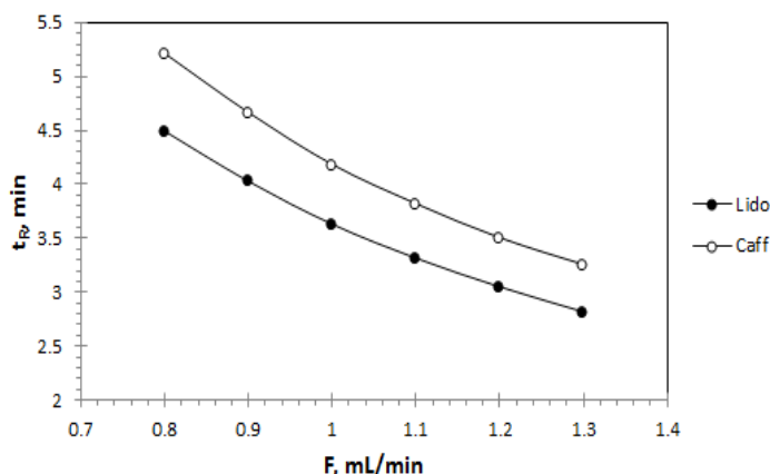
FIGURE (4): Flow rate effect of mobile phase on the retention time of (LIDO) 50 \mu\text{G/ML} AND (CAFF) 25 \mu\text{G/ML} . chromatographic conditions: C_8 column; mobile phase: acetonitrile:phosphoric acid (PH = 3) 30:70 (V/V); flow rate (VARIABLE VALUE), Temperature 30 °c and detection at 212 NM.
