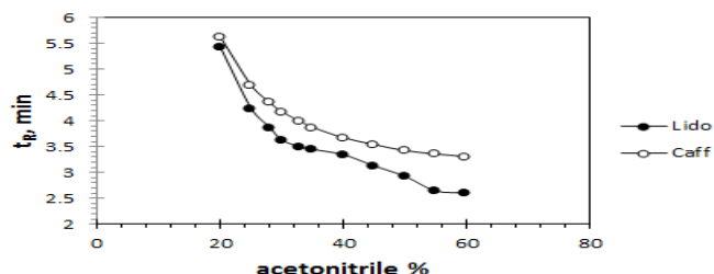
FIGURE (2): Mobile phase effect on the retention time of: (LIDO) 50 \mu\text{G/ML} and (CAFF) 25 \mu\text{G/ML} . chromatographic conditions: C_8 column; mobile phase: variable ratio of acetonitrile:phosphoric acid ( \text{pH} = 3 ), flow rate 1.0 \text{ML/MIN} , temperature 30 ^{\circ}\text{C} and detection at 212 \text{NM} .
