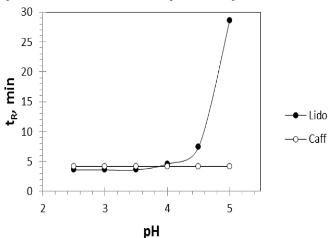
FIGURE (3): PH effect of mobile phase on the retention time ( T_R ) of (LIDO) 50 \mu\text{G/ML} and (CAFF) 25 \mu\text{G/ML} . chromatographic conditions: C_8 column; mobile phase: acetonitrile:phosphoric acid (VARIABLE VALUE OF PH) 30:70 (V/V); FLOW RATE 1.0 \text{ML/MIN} , temperature 30 ^{\circ}\text{C} and detection AT 212 \text{NM} .
