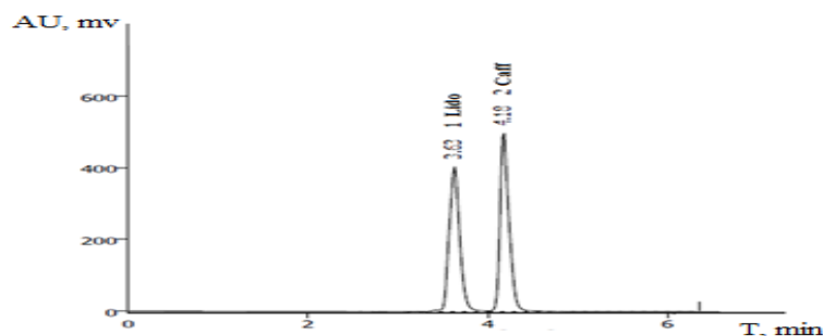
FIGURE (1): Chromatogram of standard solution: 1- (LIDO) 50 \mu\text{g/mL} , 2- (CAFF) 25 \mu\text{g/mL} . chromatographic conditions: \text{C}_8 column; mobile phase: acetonitrile:phosphoric acid ( \text{PH} = 3 ) 30:70 (V/V) flow rate 1.0 \text{mL/MIN} , temperature 30 ^{\circ}\text{C} and detection at 212 \text{NM} .
